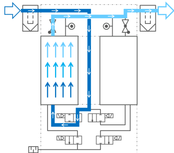
6 Adsorption - Stand-By
