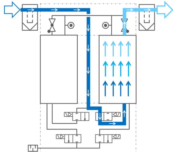
1 Stand-By - Adsorption
