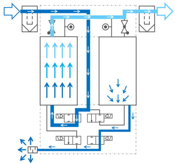
3 Adsorption - Expansion
