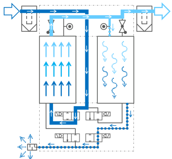
4 Adsorption – Spülen (Regeneration)
